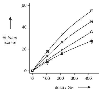
Figure 3. Dose profile of the appearance of elaidate residues (% trans isomer) from \gamma irradiation of POPC vesicles containing 60 \mu\text{M} Gly-Met and 0.2\text{M} t BuOH: ( \nabla ) \text{N}_2\text{O} -saturated natural water; ( \bullet ) \text{N}_2\text{O} -saturated 10 \text{ mM} phosphate buffer at pH 7; ( \circ ) deaerated 10 \text{ mM} phosphate buffer at pH 7; ( * ) deaerated phosphate-buffered saline (PBS); ( \square ) deaerated 10 \text{ mM} phosphate buffer at pH 6.
