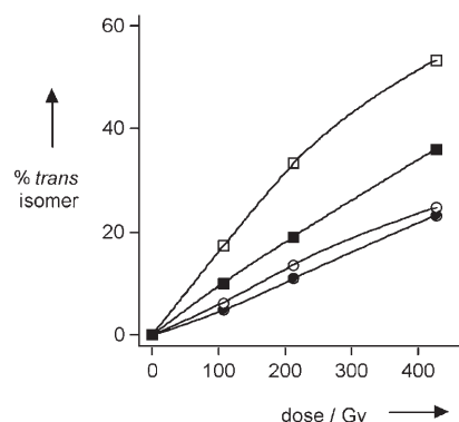
Figure 4. Dose profile of the appearance of elaidate residues (% trans isomer) from \gamma irradiation of POPC vesicles containing 60 \mu\text{M} peptide and 0.2\text{M} t BuOH in 10 \text{ mM} phosphate buffer at pH 7 and flushed with \text{N}_2 . Gly-Met ( \blacksquare ), Met-Met ( \square ), Tyr-Met ( \circ ), Trp-Met ( \bullet ).
