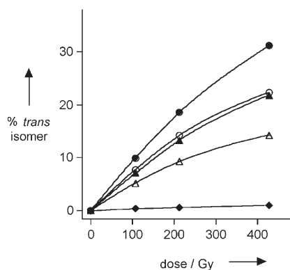
Figure 5. Dose profile of the appearance of elaidate residues (% trans isomer) from \gamma irradiation of POPC vesicles containing 60 \mu\text{M} peptide and 0.2M t BuOH in 10 mM phosphate buffer at pH 7. Met-enkephalin in deaerated ( \blacktriangle ) and \text{N}_2\text{O} -saturated ( \triangle ) solutions; Gly-Gly-Phe-Met in deaerated ( \bullet ) and \text{N}_2\text{O} -saturated ( \circ ) solutions; Leu-enkephalin in deaerated ( \blacklozenge ) solutions.
